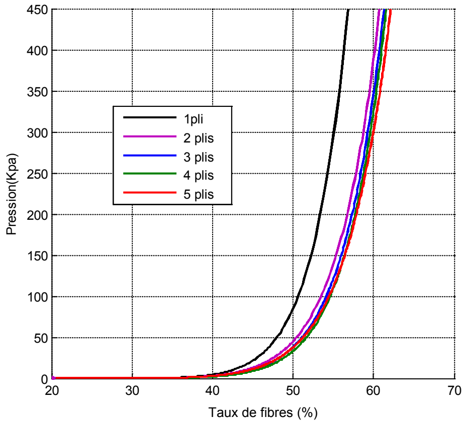
Figure 3.3 : Compression multi-plis
